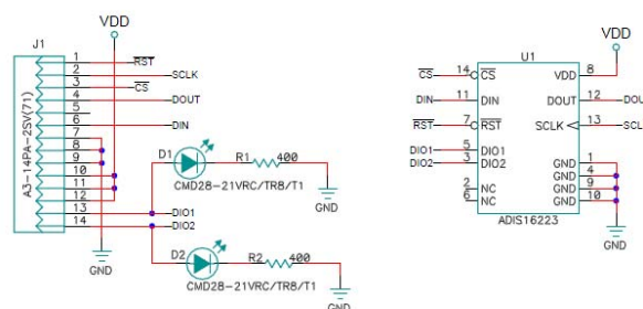
Figure 17. Electrical Schematic
